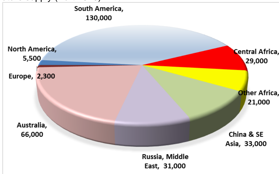
Figure 2: Estimated 'likely' resources in metric tonnes Ta 2 O 5 (after Burt 2010)
