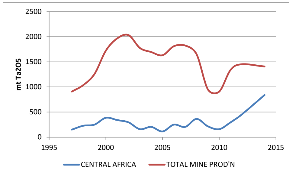
Figure 9: Mine output in metric tonnes Ta_2O_5 . Blue line: reported Central African production. Red line: total world mine production.
